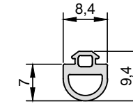
YR-0501047 BİNİ FİTLİ 5 mm STEP GASKET
