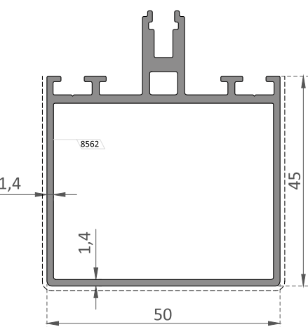
EL-1201 45 mm Yatay Profili / 45 mm Transom Profile
