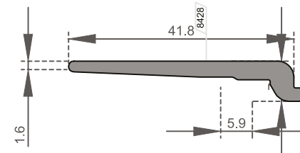
FR-5120 Cam Takoza / Glass Cleat Ağırlık / Weight 0,363 kg/m
