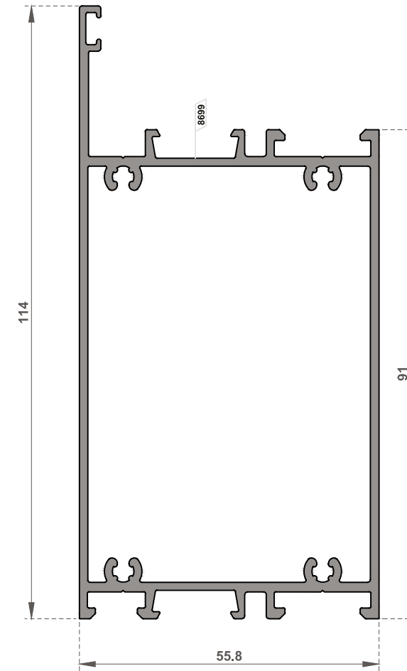
FI-4131 Sabit Baza Profili / Fix Bottom Profile
