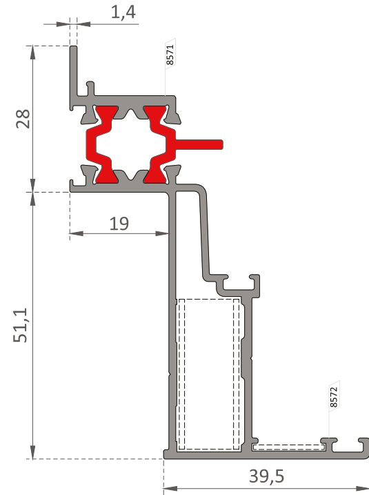
EL-1310 Kanat Profili / Sash Profile
