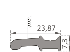
EL-2122 Kitleme Profili / Interlocking Profile
