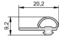
YR-0501055 Kanat Bini Fitili Sash Step Gasket
