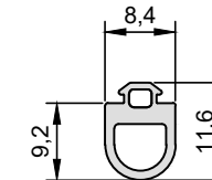
YR-0501048 BİNİ FİTLİ 7 mm STEP GASKET
