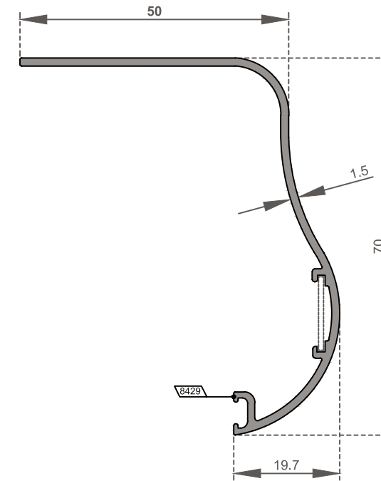
OM-5420 Dekoratif Pervaz Profili / Decorative Arcitrave Profile Ağırlık / Weight 0,558 kg/m
