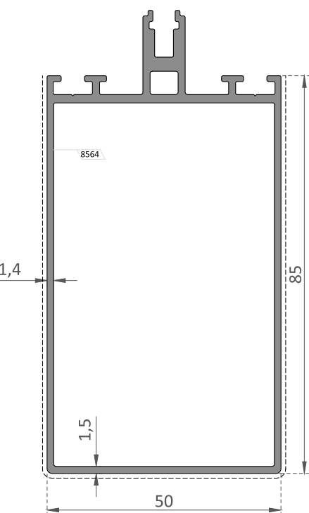
EL-1203 85 mm Yatay Profili / 85 mm Transom Profile
