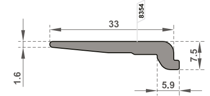
OM-5120 Cam Takoza / Glass Cleat
