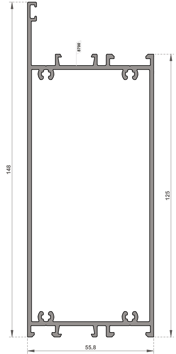
FI-4132 Sabit Baza Profili / Fix Bottom Profile
