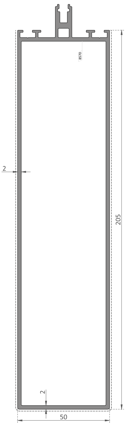
EL-1220 205 mm Yatay Profili / 205 mm Transom Profile
