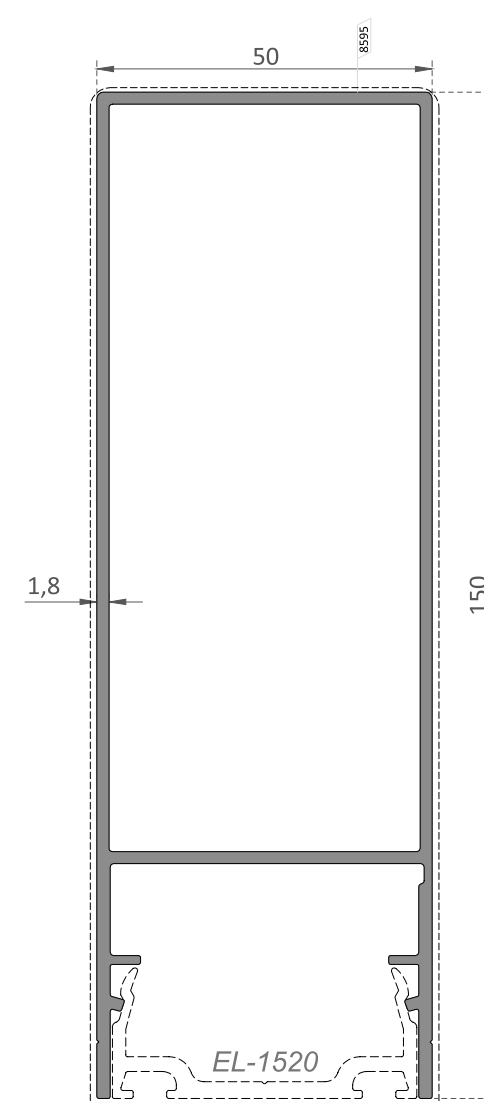
EL-1625 150 mm Kapak Profili / 150 mm Cover Profile
