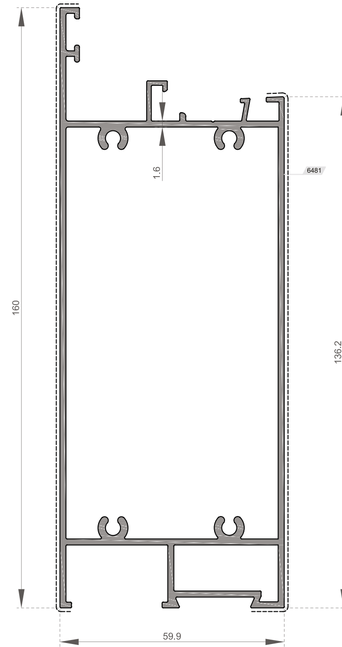
PA-4250 Etek Profili 136.2/160 / Buttom Plate Profile 136.2 / 160 Et Kalınlığı / Wall Thickness 1.6mm
