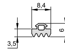
YR-0501046 DİŞ CAM FİTLİ 3 mm OUTER GLAZING GASKET
