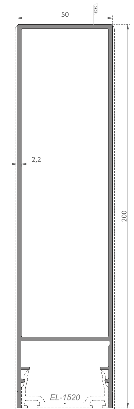
EL-1626 200 mm Kapak Profili / 200 mm Cover Profile
