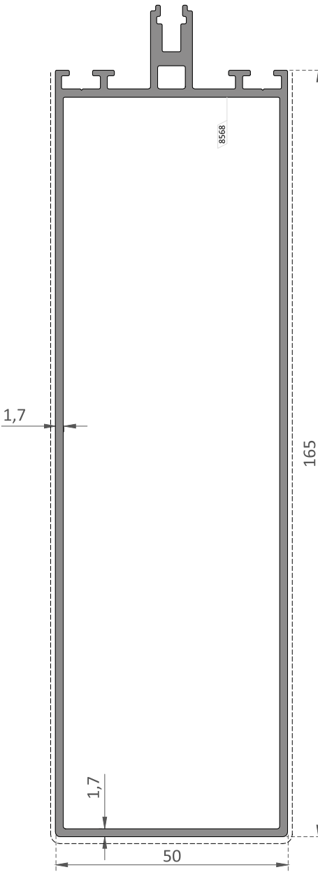
EL-1214 165 mm Yatay Profili / 165 mm Transom Profile
