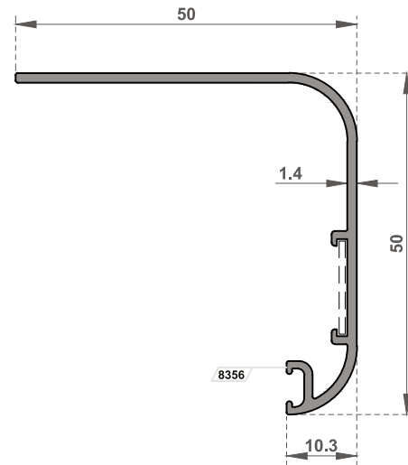
OM-5411 Dekoratif Pervaz Profili / Decorative Architrave Profile
