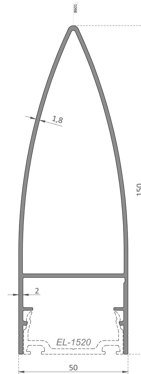
EL-1633 150 mm Dekoratif Kapak Profili / 150 mm Decorative Cover Profile
