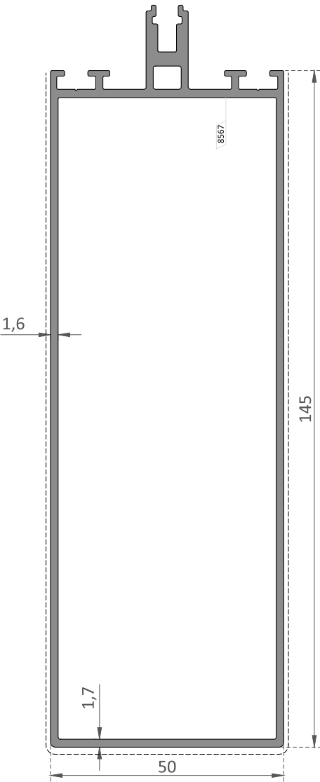
EL-1213 145 mm Yatay Profili / 145 mm Transom Profile
