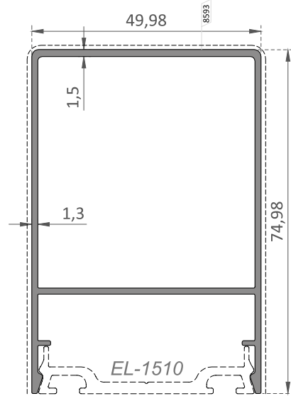
EL-1623 75 mm Kapak Profili / 75 mm Cover Profile
