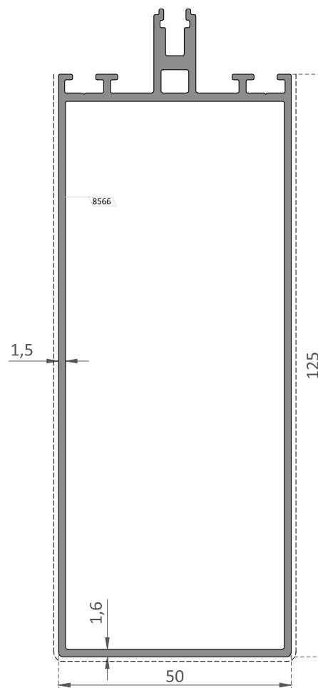
EL-1212 125 mm Yatay Profili / 125 mm Transom Profile
