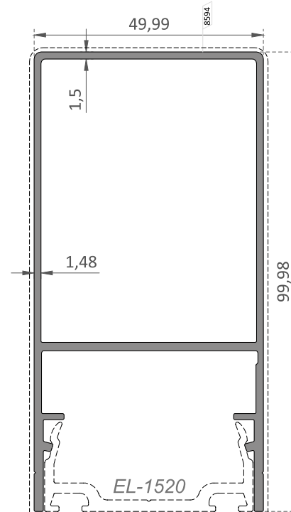
EL-1624 100 mm Kapak Profili / 100 mm Cover Profile
