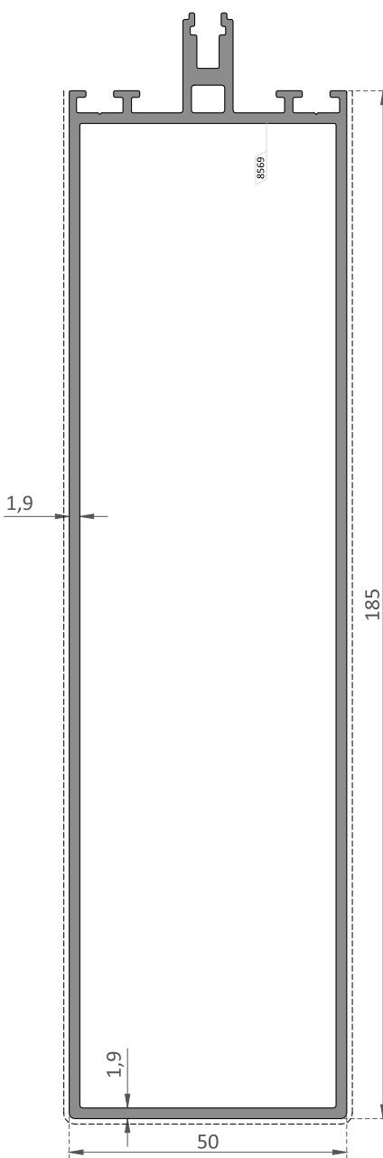
EL-1215 185 mm Yatay Profili / 185 mm Transom Profile
