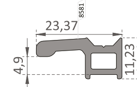
EL-2121 Kitleme Profili / Interlocking Profile
