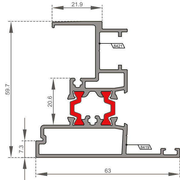
FS-2630 PVC Kanallı Çift Kanat Adaptör Profili / Double Sash Adapter Profile With PVC Groove Ağırlık / Weight 1,291 kg/m
