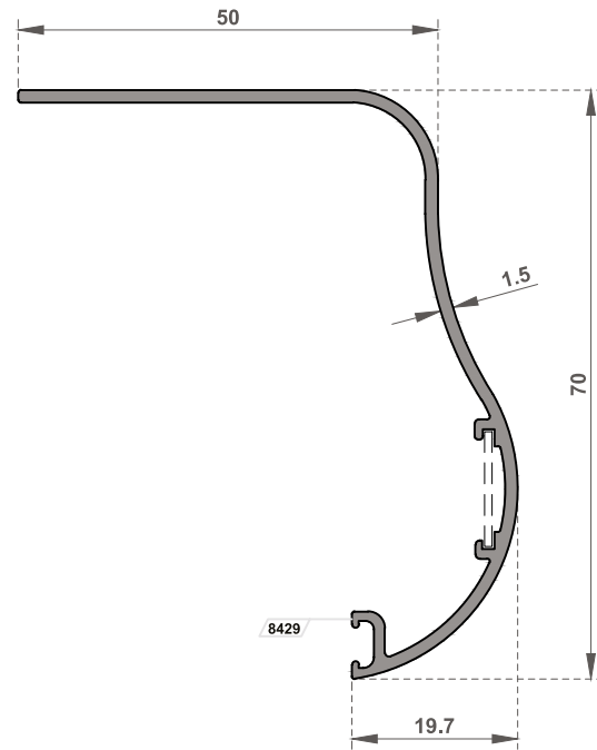
OM-5420 Dekoratif Pervaz Profili / Decorative Architrave Profile
