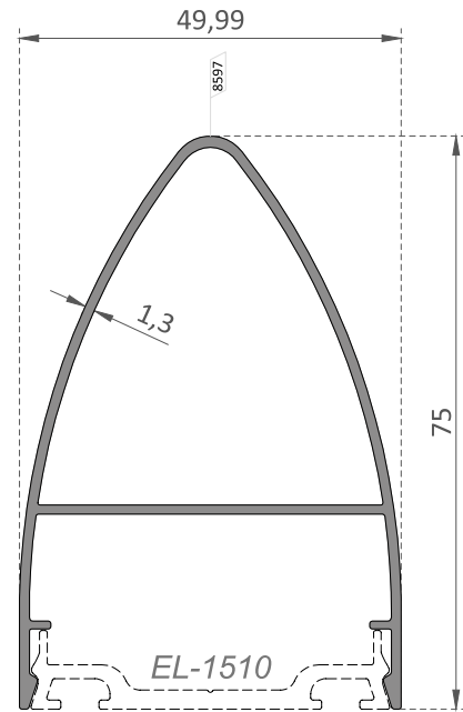
EL-1631 75 mm Dekoratif Kapak Profili / 75 mm Decorative Cover Profile
