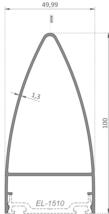
EL-1632 100 mm Dekoratif Kapak Profili / 100 mm Decorative Cover Profile
