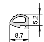
YR-0501049 KAMA FİTLİ 3.5 mm GLAZING GASKET
