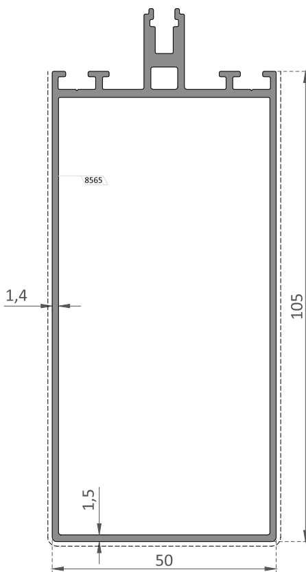
EL-1211 105 mm Yatay Profili / 105 mm Transom Profile
