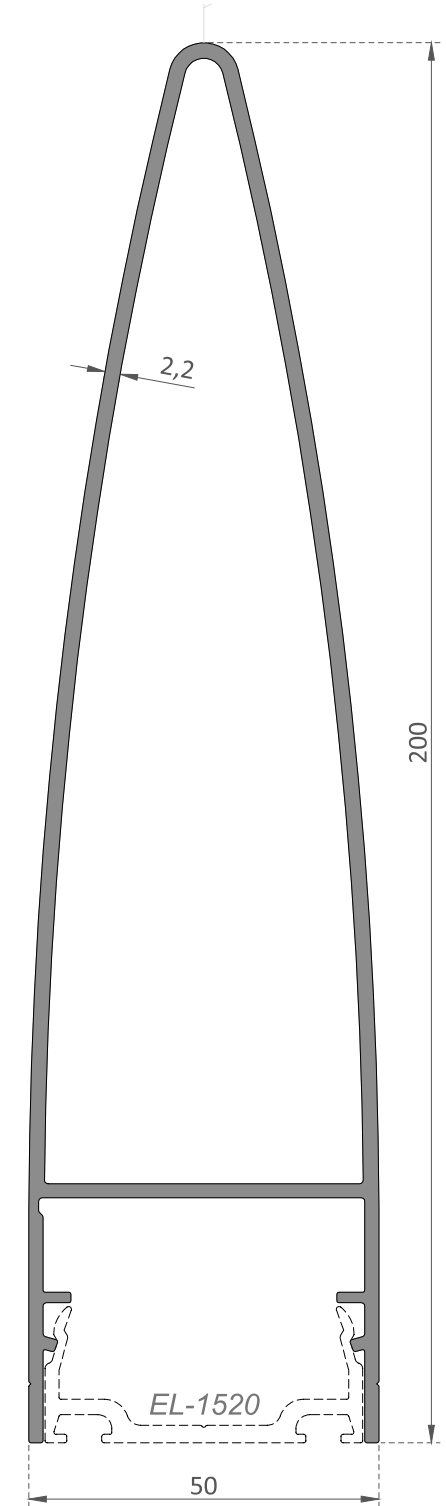
EL-1634 200 mm Dekoratif Kapak Profili / 200 mm Decorative Cover Profile
