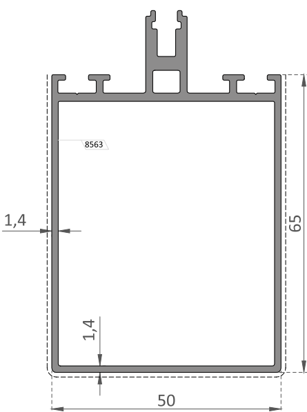
EL-1202 65 mm Yatay Profili / 65 mm Transom Profile
