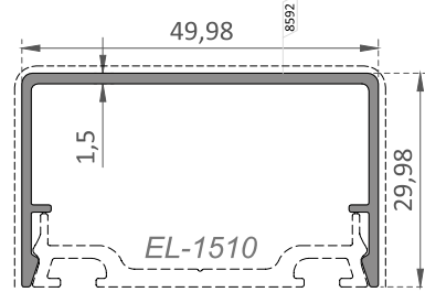
EL-1621 30 mm Kapak Profili / 30 mm Cover Profile
