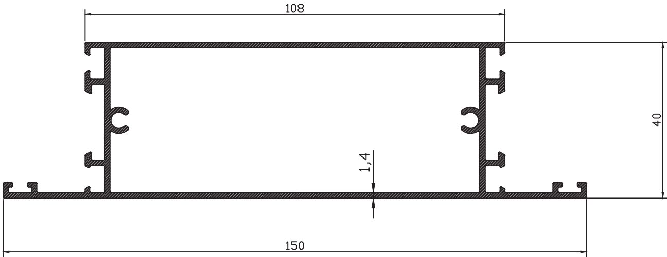
ER-7744 1,547 kg/m
