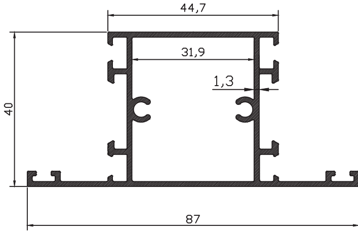
ER-7726 1,002 kg/m
